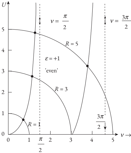
Fig. 3.8a “Even” solutions occur at the intersection of curves represented by u = v \tan(v)
