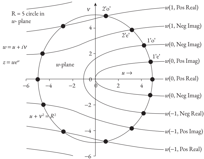
Fig. 3.13 Maps in the w plane of the axes-rays in the z plane, using the Lambert W function. The notation w(k, \text{ray}) which labels the curves in the w plane specifies the k^{\text{th}} branch, and the specific ray specified. The four solutions in the quadrant for (u > 0, v > 0) are labeled as 1'e' , 1'o' , 2'e' , and 2'o' corresponding to the 1st and 2nd “even” ( \varepsilon = +1 ) and “odd” ( \varepsilon = -1 ) solutions of Fig. 3.8.
