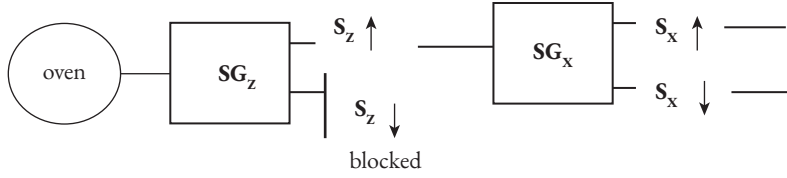
Fig. 1.2c Selected output of the first SG experiment in which the magnetic field is along the z -axis is input to a second SG apparatus in which the magnetic field is orthogonal to that in the first.
