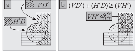
Fig. 11.3 The sets H' and D' denote the complements of H and D respectively. The intersection H'D = H' \cap D of H' and D is shaded with dashes sloping left to right upward, while the intersection VD' = V \cap D' of V and D' is shaded with dashes left to right sloping downward. The intersection VH' = V \cap H' of V and H' is shown with stars (asterisks).
