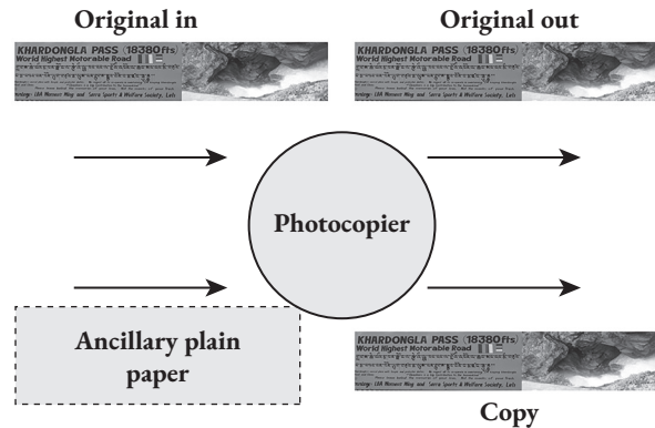
Fig. 11.12 A photocopier accepts as input any document or image along with an ancillary blank sheet of plain paper and delivers the original unaltered and a copy of the same.
