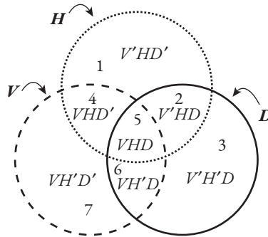
Fig. 11.4 Each of the three circles H (dotted line for circumference), V (dashed line for circumference), and D (continuous line for circumference) partly overlaps with the other two circles. The circle H has a part that overlaps with circle V and a part that does not. It also has a part that overlaps with the circle D and a part that does not. The circles V and D also have similar relationships with the other two circles.
