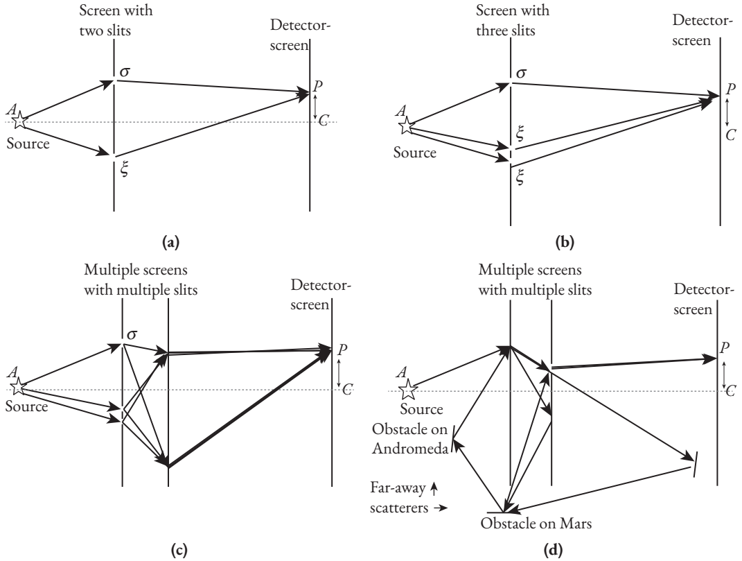
Fig. 2.2 The four panels in this figure, (a) through (d), show a gedanken Young's interference experiment in which the experimental setup allows increasingly zigzag paths, no matter how bizarre they seem to be, which FP can take from its source to a destination point on the detector-screen.
