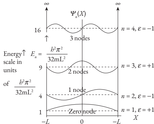
Fig. 3.9 Energy levels and corresponding wavefunctions of a particle confined in an impenetrable potential barrier. Observe the nodal structure in conformity with the separation theorem and the comparison theorem discussed in the text.
