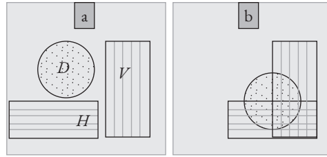
Fig. 11.2 The panel [a] on the left shows Venn diagrams for a set H (rectangle with horizontal stripes), a set V (rectangle with vertical stripes), and a third set D (a dotted circle). The panel [b] on the right shows these three sets displaced and arranged such that parts of D , H and V overlap with each other, constituting partial intersections that we shall denote by \cap .
