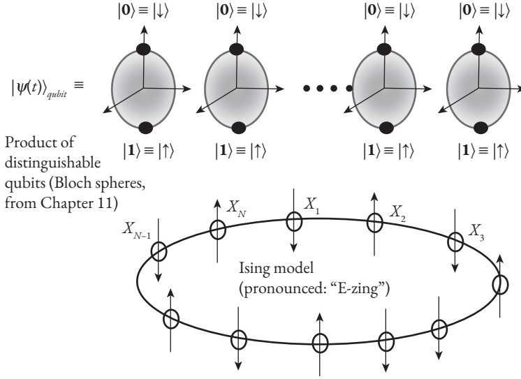
Fig. E.1 Distinguishable qubits, numbered like spins in an Ising model.
