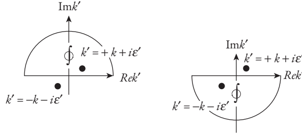
Fig. 10.13 This contour integration path includes the entire real axis. The poles are avoided by displacing them infinitesimally and then taking the limit as the magnitude of the displacement tends to zero.
