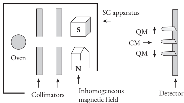
Fig. 1.2a Stern–Gerlach experiment. Collimated silver atoms pass through an inhomogeneous magnetic field along the z -axis. Classical mechanics predicts a single spot at the centre of the detector in line with the collimated beam. Quantum mechanics predicts two separated spots, as are actually observed in the SG experiment. One spot is above the centre, and the other is symmetrically below it.
