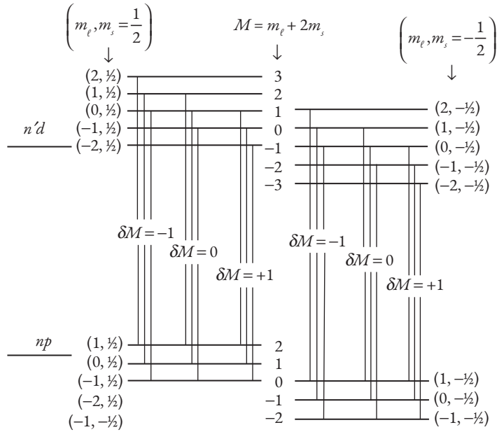
Fig. 8.8a The electric dipole transition n'd \rightarrow np splits into nine transitions for m_s = +\frac{1}{2} and also for m_s = -\frac{1}{2} . However, only three frequencies are observed in the spectrometer since the splitting of the energy levels is equispaced.
