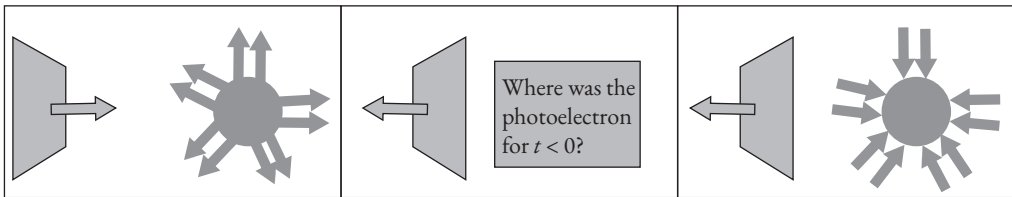
Fig. 10.4 The left-most panel depicts a scattering experiment in which a monoenergetic beam of incident particles impinging on a target is scattered away in various directions by the target. The right-most panel shows a photoelectron that escapes away to the asymptotic region as a free particle, but since it did not exist as a free particle in the initial state, it must be depicted by incoming spherical waves, in which the incoming flux from any direction is canceled from that coming in from the opposite side.
