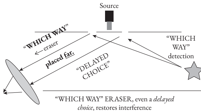
Fig. 3.3c In this setup, the eraser is placed far away. However, regardless of where the eraser is placed, close by or far away, the mere provision of an eraser restores interference.
