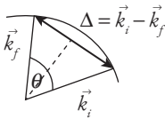
Fig. 10.15a Change in momentum in collision.
