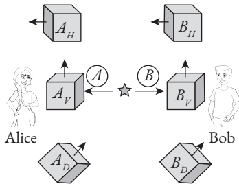
Fig. 11.5a The top row, middle, and the bottom row depict three pairs of Stern–Gerlach (SG) basis sets, with Alice and Bob. The direction of the SG magnetic field (axis of quantization) in the three pairs of apparatus is different. Alice and Bob may choose to perform experiment in any of the three basis sets of SG apparatus.
