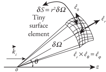
Fig. 10.1d A tiny surface element \delta S on the shaded curved strip (on the spherical surface) shown in Fig. 10.1c subtends a solid angle \delta \Omega at the center of the scatterer.
