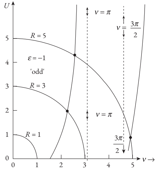
Fig. 3.8b “Odd” solutions occur at the intersection of curves represented by u = -v \cot(v)
