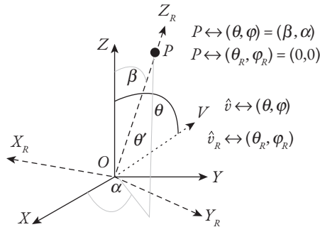
Fig. 4.3 With a common origin O , we have a Cartesian coordinate frame of reference (X_R, Y_R, Z_R) that is rotated with respect to (X, Y, Z) . The polar and azimuthal coordinates of an arbitrary point on the line OV along the direction given by the unit vector \hat{v} = \hat{v}_R are (\theta, \varphi) with respect to the frame (X, Y, Z) and (\theta_R, \varphi_R) with respect to (X_R, Y_R, Z_R) . The polar coordinates of a point P on the Cartesian axis Z_R are (\theta, \varphi) = (\beta, \alpha) with respect to the frame (X, Y, Z) and (\theta_R, \varphi_R) = (0, 0) with respect to (X_R, Y_R, Z_R) . We shall denote a unit vector along the axis Z_R by \hat{u} .
