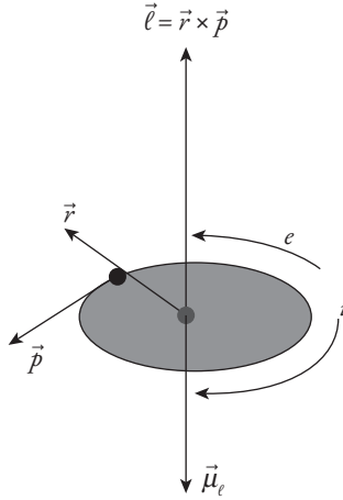
Fig. 7.2 This is a semi-classical model of an electron circling a proton in the hydrogen atom. The electron's instantaneous position with respect to the nucleus is \vec{r} , instantaneous kinetic momentum is \vec{p} , and the orbital angular momentum is \vec{\ell} . This motion can be likened to an electric current i = \frac{e}{T} = e \frac{v}{2\pi r} , where e is the electron's charge, v its speed, and T the time period for one full rotation. Associated with this current is then a magnetic dipole moment \vec{\mu}_\ell = \frac{1}{c} i A \hat{A} = \frac{1}{c} \left( e \frac{v}{2\pi r} \right) (\pi r^2) \hat{A} = \frac{1}{c} \frac{evr}{2} \hat{A} , i.e., \vec{\mu}_\ell = \frac{e}{2c} \vec{r} \times \vec{v} = \frac{e\hbar}{2mc} \frac{\vec{\ell}}{\hbar} .
