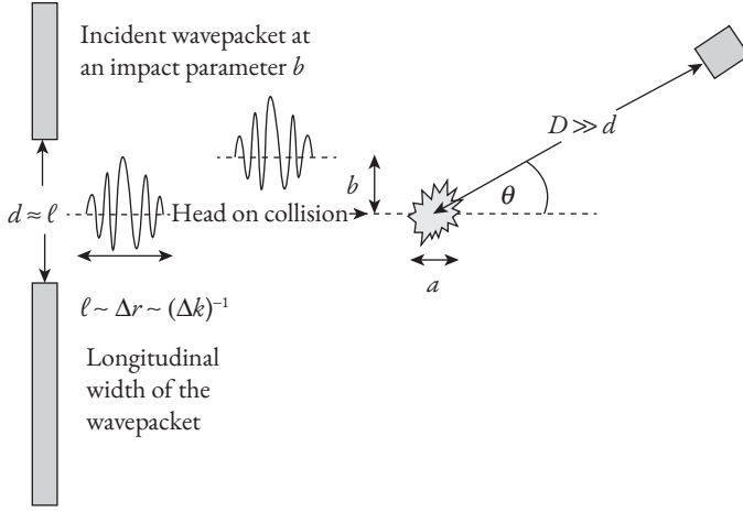
Fig. 10.1a Schematic diagram showing scattering of an incident beam of probe particles by a target scatterer. We assume that the transverse width d is about the same as the wavepacket's longitudinal width.
