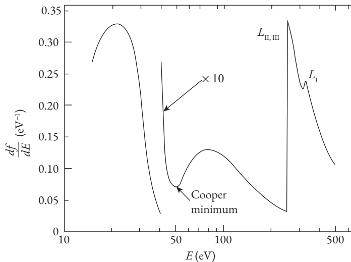
Fig. 8.1 The change in sign of the matrix elements (Eq. 8.26) makes the photoionization cross-section go through a zero at some energy, called as the Cooper minimum . It is illustrated here, with permission from Reference [2]. The delayed maximum in the photoionization cross section is also seen in this figure.
