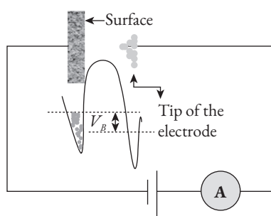
Fig. 3.5a The inset of this figure shows a schematic representation of the potential function.
