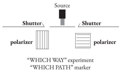
Fig. 3.2a A WW marker destroys interference. The detector screen is represented in this figure by the straight line at the bottom.
