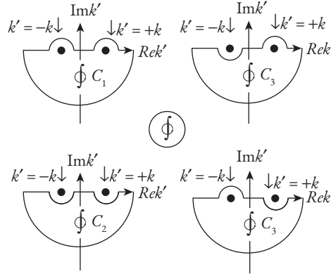
Fig. 10.12 Four different paths of integration for the evaluation of the integral I_2 (Eqs. 10.165a,c). The choice C_2 gives zero; the remaining three choices correspond to different boundary conditions listed in Table 10.2.
