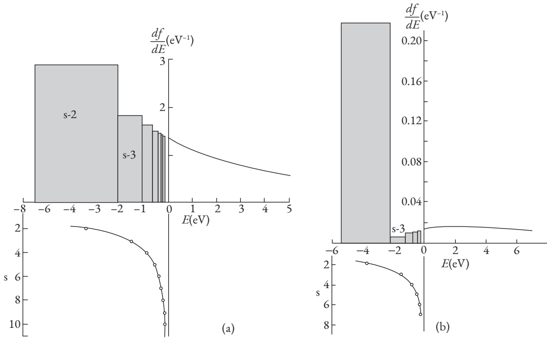
Fig. 8.3 Oscillator strength distributions (reproduced with permission from Ref. [2]) in the discrete and the continuous spectra of (a) H (theory) and (b) Li (experiment). Oscillator strengths for discrete transitions are plotted as histogram blocks of height \frac{f_s}{\Delta E} , where the base of each block is determined by the geometrical construction of tangents to the \dot{E}_s versus s curve as shown in the lower part of (a).
