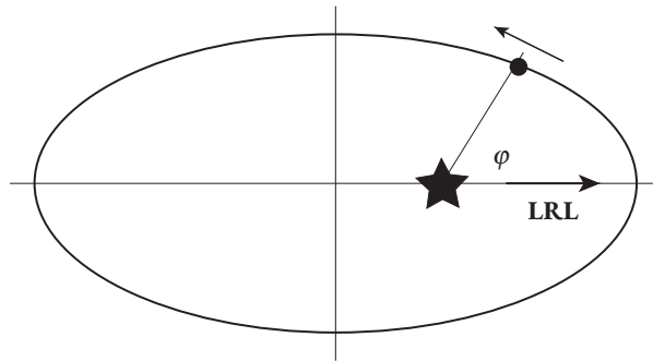
Fig. 5.6 The classical Laplace–Runge–Lenz vector points from the focus to the perigee. It is a constant vector for the one-over-distance potential. It keeps the major axis fixed; prevents its precession.
