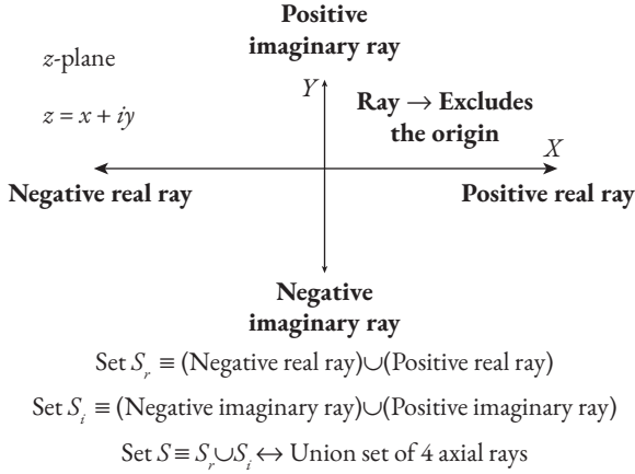
Fig. 3.11a The complex z plane.
