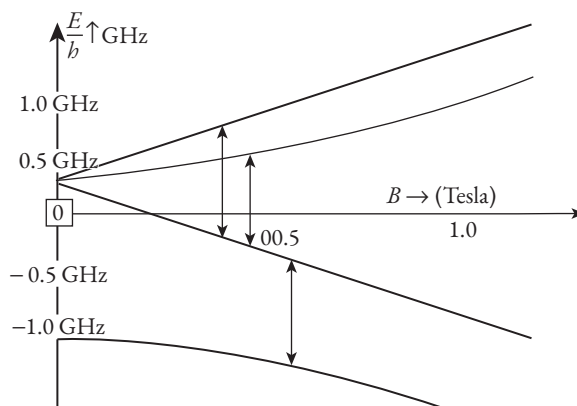
Fig. 8.11b M_JM_I are no longer good quantum numbers due to \vec{J} \cdot \vec{I} coupling. The eigenstates of the Hamiltonian are now given by superposition of |M_JM_I\rangle base vectors. Figure adapted from Reference [20].
