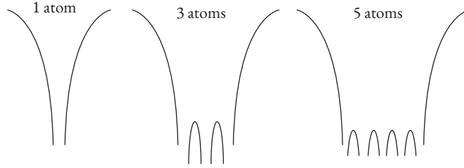
Fig. 3.7a Atomic potentials in a nanostructure.
