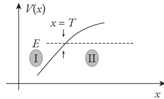
Fig. 6.1b Region I is classically allowed (CA); region II is forbidden. The classical turning point is at x = T .
