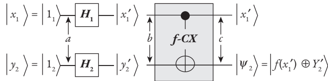
Fig. 11.10 In the DJ algorithm, two single qubits each in pure state |1\rangle are input to two 1qb Hadamard gates H_1 and H_2 . The outputs from the two H gates are fed to the 2-qubit f -CX function box.
