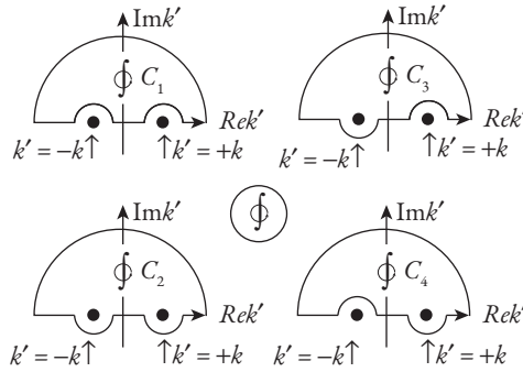
Fig. 10.11 The closed paths C_1 , C_2 , C_3 and C_4 , show four different ways to choose the path of integration for the evaluation of the integral I_1 (Eqs. 10.165a,b). The choice C_1 gives zero, and the remaining three choices correspond to different boundary conditions listed in Table 10.1.
