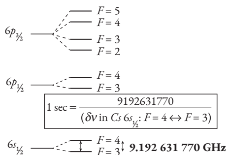
Fig. 8.12 Transition between F=4 and F=3 levels of the 6s hyperfine levels ^{133}\text{Cs} , which defines the unit of time.
