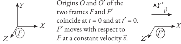
Fig. 7.1 Two Cartesian inertial frames of references with their respective axes parallel to each other and moving at a constant velocity \vec{v} with respect to each other.
