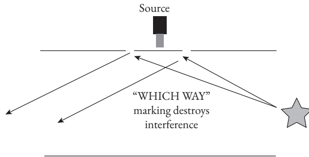
Fig. 3.3a As in Fig. 3.2, the detector screen is represented in this figure by the straight line at the bottom. Shining light behind the slits to peek into the path is another way of conducting a WW experiment. This serves as a WW marker. WW marking destroys interference.
