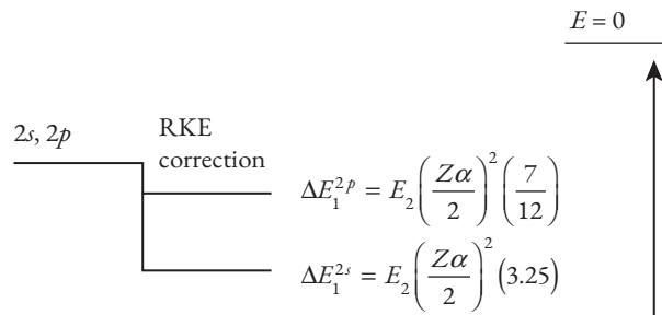
Fig. 7.4 The relativistic kinetic energy correction to the energy level depends on the value of the orbital angular momentum quantum number.
