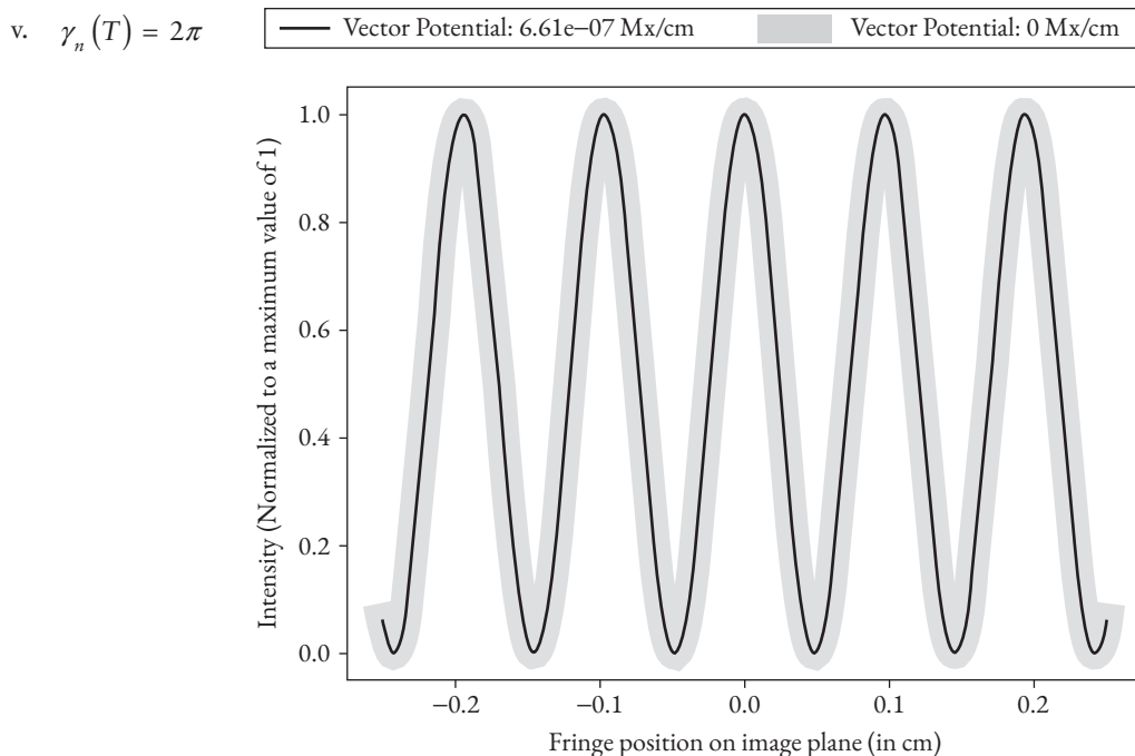
Fig. 2.6 Displacement of the fringes due to the Aharonov–Bohm effect respectively for the five cases tabulated in Table 2.1. There is a lateral displacement as the geometric phase increases. The thick curve for “no current” is included in each to provide reference for the relative displacement. The similarity of the pattern in (i), (iii), and (v) is only apparent as the displaced fringes fall on top of adjacent ones as the geometric phase changes. The same is true for (ii) and (iv).
