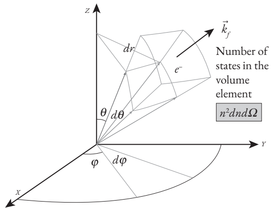
Fig. 6.6b Determination of the number of states into which the photoionization transition can take place.
