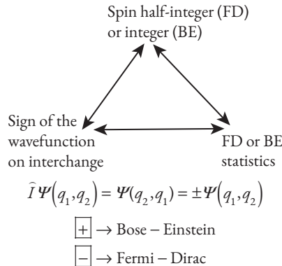
Fig. 9.1 The relationship between symmetry of the N -particle wavefunction, value of the intrinsic spin angular momentum quantum number, and the statistical distribution function.
