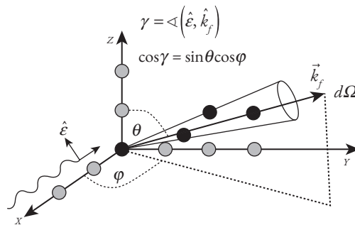
Fig. 6.5 The electromagnetic radiation is considered to be polarized along the direction \hat{\epsilon} and incident along the x -axis. The photoelectron is ejected along \hat{\epsilon} = \hat{k}_f .
