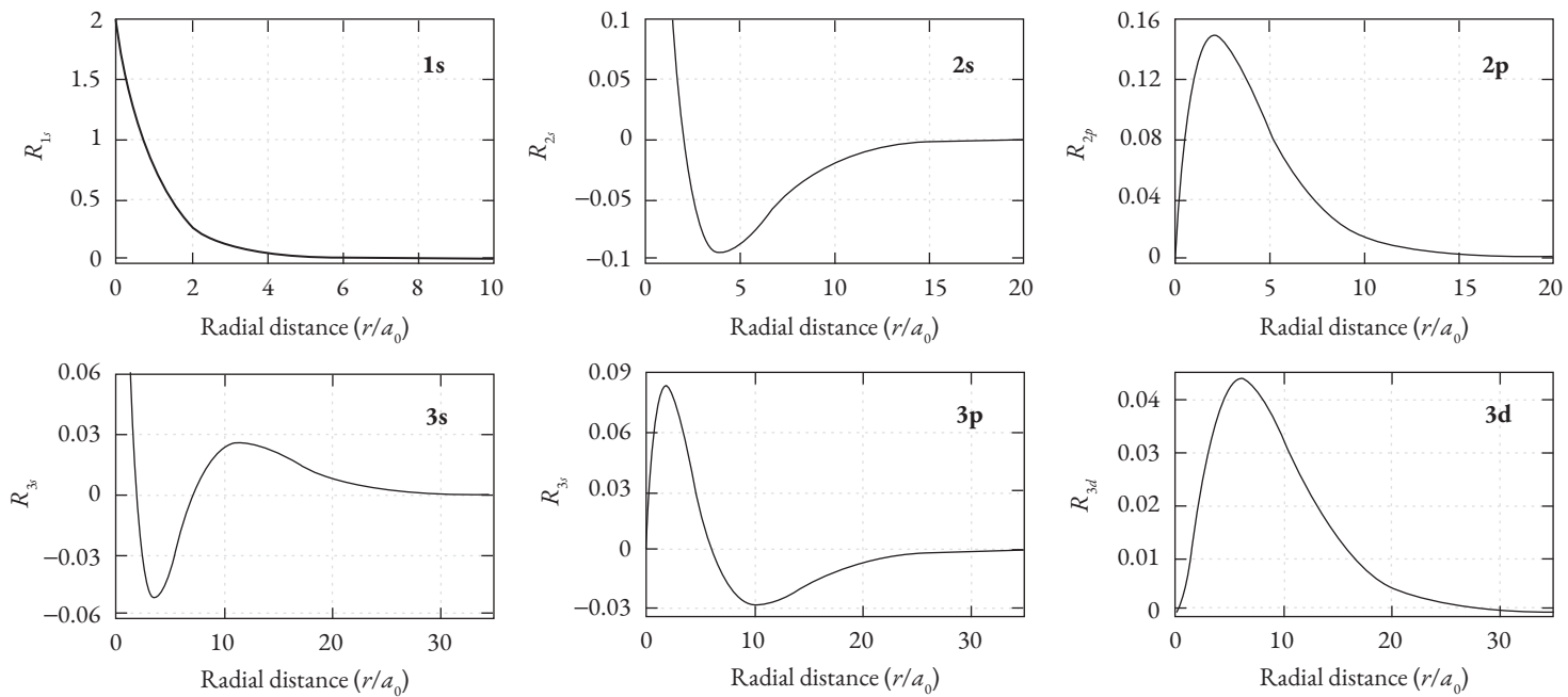
Fig. 5.4 Illustrative radial wave functions of the hydrogen atom. Figures plotted by Nishita Manohar Hosea.
