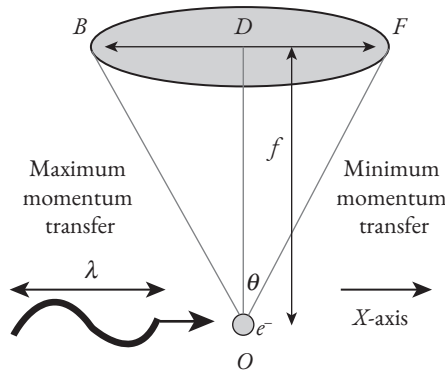
Fig. 1.1 The Heisenberg microscope is an apparatus we employ to discuss a thought experiment that demonstrates that accuracy in the measurement of an object's position is inversely related to that in a concurrent measurement of its momentum.
