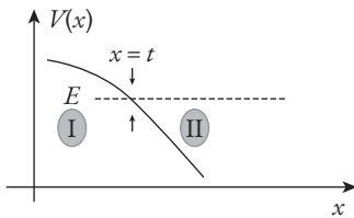
Fig. 6.1a Region I is classically forbidden (CF); region II is allowed. A particle described by classical physics can be found only in the region II, to the right of x = t , where E > V .
