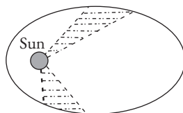
Fig. 4.1 Our perception of angular momentum is built on the basis of classical models such as the Kepler–Newton planetary orbits.
