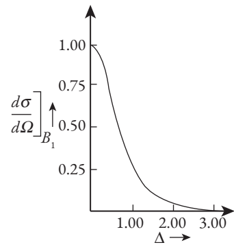
Fig. 10.15c Angular anisotropy of the differential cross section in the first Born approximation. Adapted from Chapter 8 of Reference [3].
