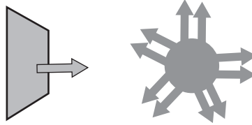
Fig. 10.2c Schematic diagram showing a plane wavefront incident on a target scattering center. The scattered wave would travel radially outward after scattering, but the scattering yield can be anisotropic.
