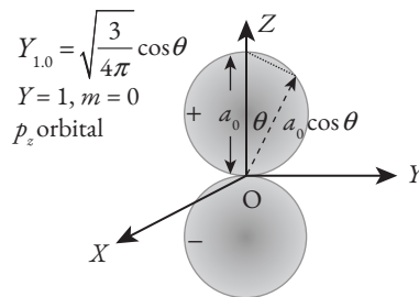
Fig. C.2 The atomic p_z orbital is shaped in the figure of 8, rotated about the Z -axis through one full circle. The lobes above and below the XY -plane are perfectly spherical. Since the diameter of a circle subtends an angle of 90^\circ at any point on the circumference, the side of the triangle shown by dashed lines scales as a_0 \cos \theta , as shown, corresponding to the Legendre polynomial for \ell = 1 , m = 0 .
