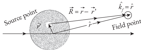
Fig. 10.9 Schematic representation of the cause-effect relationship depicting the influence at the field point of the extended source of inhomogeneity in the differential equation. Whole space integration over the extended region of the source must be carried out to get the cumulative effect at the field point.
