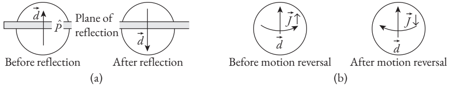
Fig. A.4 Under parity transformation, the angular momentum remains invariant, but the electric dipole moment would reverse sign. Under the time-reversal operation, just the opposite would happen.
