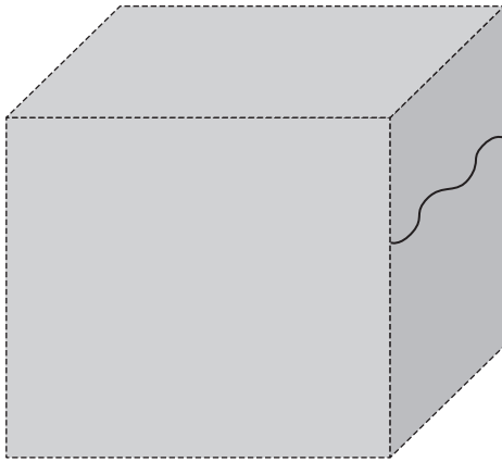
Fig. 6.6a Box normalization relies on determining that wavelengths can be sustained in the box since only an integer multiple of the wavelengths can do so. Therefore, the following relations hold:
