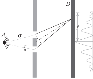
Fig. 2.5a Phase difference between alternative paths produces interference through superposition.
