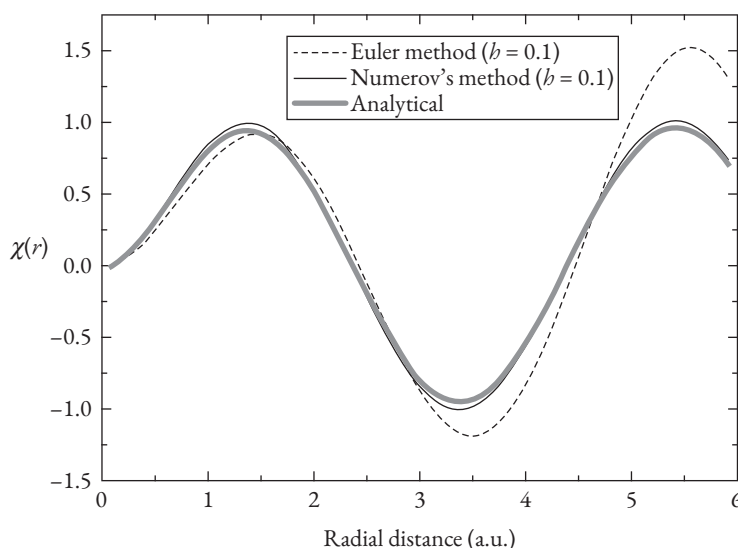
Fig. P6.11 Comparison of radial wavefunction obtained using the Euler (black dashed) and Numerov's method (black solid) and analytical function (thick grey).
