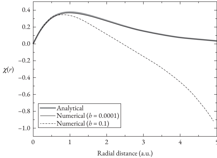
Fig. P6.10 Comparison of radial wavefunction obtained using the Euler equation ( h = 0.0001 : black solid, h = 0.1 : black dashed) and analytical function (thick grey).
