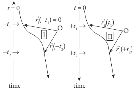
Fig. A.3 Depiction of the time-reversal symmetry in classical laws of motion.
