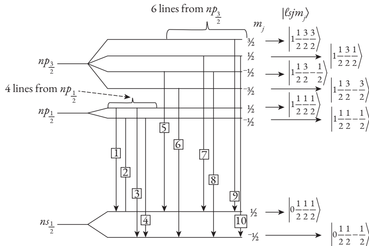
Fig. 8.9 The d_1 and d_2 lines of the sodium atom split into 10 lines.
