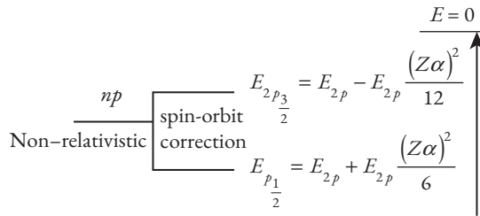
Fig. 7.3 Spin-orbit splitting of the 2p level in the hydrogen atom. Note that the 2p_{\frac{3}{2}} level is less negative, and the 2p_{\frac{1}{2}} level is more negative than the energy of the nonrelativistic 2p level.
