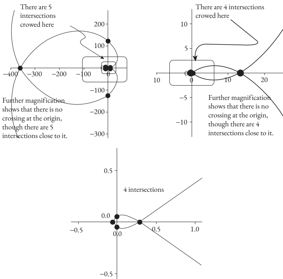
Fig. 3.12 Image of the R -circle in w plane gives closed multi-loop self-intersecting curve, which is referred to as the Q -curve in the z plane. Solutions to the FSW (finite square well) problem are given by the points of intersection of the Q curve in the z plane with the coordinate axes. On successive magnification shown in the three panels below of the portion in the rectangle near the origin, one can see that the Q curve crosses the axes 14 times.
