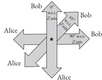
Fig. 11.5b When Alice chooses V , Bob may choose H or V or D . They pick their apparatus without consulting each other. Likewise, when Alice chooses H , Bob may independently choose H or V or D , etc. Their findings are examined after all experiments are performed [2].
