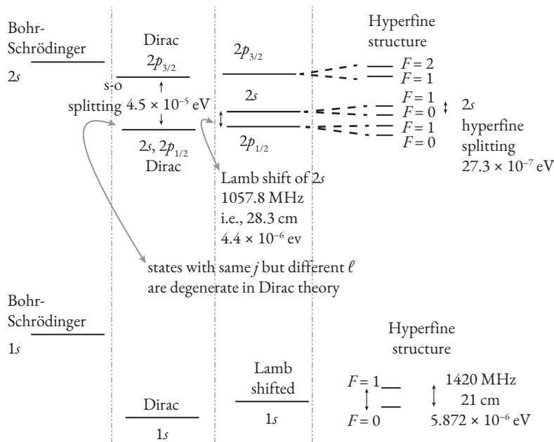
Fig. 7.5 Bohr–Schrödinger energy levels in the nonrelativistic energy spectrum of the hydrogen atom shift due to relativistic effects. RKE lowers the energy levels; spin–orbit interaction splits energy levels of j = \ell \pm \frac{1}{2} . The Darwin correction affects only the \ell = 0 states. The three corrections, s-o, RKE, and Darwin, are intrinsically present in Dirac theory; the FW transformations bring them to the surface and make them manifest. The energy levels are further shifted, due to factors not accounted for in Dirac theory. These additional shifts are the Lamb–Retherford shift and shift on account of the hyperfine structure.
