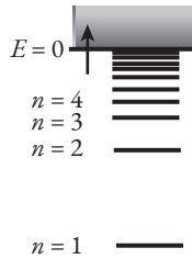
Fig. 5.2 Schematic diagram of the energy levels of the hydrogen atom modeled by the Schrödinger equation. The bound states energy eigenvalues are given by Eq. 5.47. The energy eigenvalues turn out to be exactly the same as in the Rydberg-Balmer semi-empirical model, and also the Bohr-model of the old quantum theory. Bound states ( E < 0 ) have a discrete spectrum, and unbound states ( E > 0 ) have a continuum.
