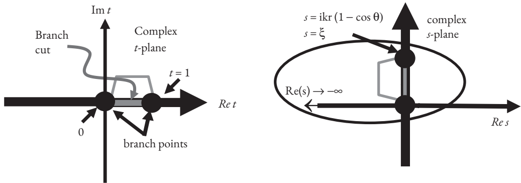
Fig. 5.7 a, b The left panel in this figure shows the branch points in the complex t plane and the right panel shows the same in the complex s plane. The flexed branch cut is also shown.
