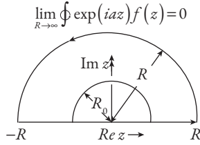
Fig. 10.10 For a function f(z) that is analytic in the upper half of the complex plane in the region |z| > R_0 , and \lim_{R \rightarrow \infty} |f(z)| \rightarrow 0 then \lim_{R \rightarrow \infty} \oint \exp(iaz) f(z) = 0 (for a > 0 ); the path integral being over the large semicircle. When a < 0 , the integration must be over a similar semi-circle in the lower half of the complex plane. This is a widely used result in complex analysis known as the Jordan's lemma.
