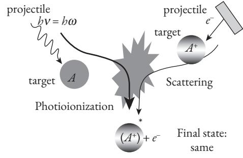
Fig. 10.2b The final state of photoionization ( h\nu + A \rightarrow A^{+*} + e ) and electron-ion scattering ( A^+ + e \rightarrow A^{+*} + e ), are the same, even though the initial ingredients of the reaction are different. These two processes are related by time-reversal symmetry.
