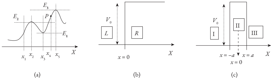
Fig. 3.4 The analysis of one-dimensional motion along the x -axis is different in classical mechanics and in quantum mechanics. (a) A particle on a one-dimensional roller coaster. (b) A step potential. The potential is zero for x < 0 and it is V_0 for x > 0 , all the way as x \rightarrow \infty . (c) A potential that is zero for x < -a (region I), V_0 in region between x = -a and x = +a (region II), and zero again in region x > a (region III).
