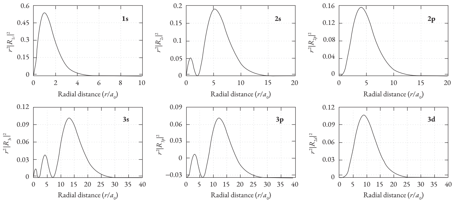
Fig. 5.5 Plots of radial probability densities corresponding to the functions shown in Fig. 5.4. Figures plotted by Nishita Manohar Hosea.
