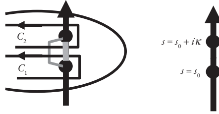
Fig. 5F.1 a, b The left panel (a) shows the choice of contour to address the branch points in the complex s plane. The flexed branch cut is also shown. The right panel (b) shows that for each point on the curve C_1 , there is a corresponding point directly above it on C_2 at a distance (i\kappa) .
