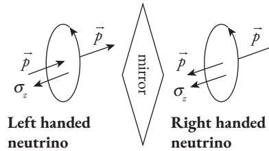
Fig. A.2b A mirror image of the left-handed neutrino would produce the right-handed neutrino; but the latter has not been ever detected.
