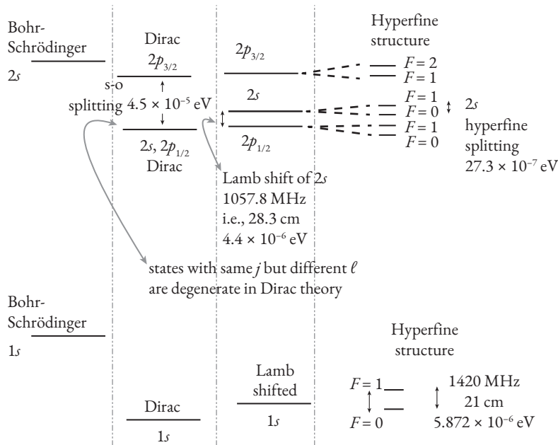
Fig. 8.10 Bohr-Schrödinger energy levels in the nonrelativistic energy spectrum of the hydrogen atom shift due to relativistic effects. RKE lowers the energy levels; spin-orbit interaction splits energy levels of j = \ell \pm \frac{1}{2} . The Darwin correction affects only the \ell = 0 states. The energy levels are further shifted due to factors not accounted for in Dirac theory. These additional shifts are the Lamb-Retherford shift, and shift on account of the hyperfine structure. This diagram is of course only schematic, not to scale.
