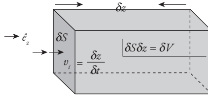
Fig. 10.6 Estimation of the correspondence between the probability current density and the density of projectile particles.
