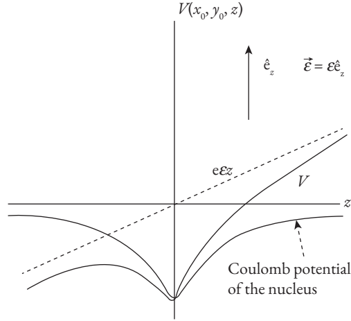
Fig. 8.4 Schematic diagram showing the effective potential experienced by an electron in the hydrogen atom placed in a constant electric field.
