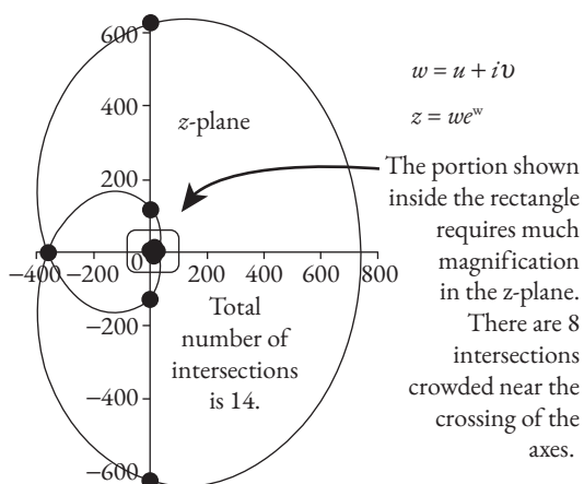
Fig. 3.12 Image of the R -circle in w plane gives closed multi-loop self-intersecting curve, which is referred to as the Q -curve in the z plane. Solutions to the FSW (finite square well) problem are given by the points of intersection of the Q curve in the z plane with the coordinate axes. On successive magnification shown in the three panels below of the portion in the rectangle near the origin, one can see that the Q curve crosses the axes 14 times.
