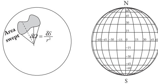
Fig. 2.7 The figure on the left shows a closed curve on a sphere along which a pendulum can be parallel and transported adiabatically. The figure on the right shows that a pendulum set in motion, say somewhere in the northern hemisphere of the earth, would begin its oscillation in a certain plane to which it would not return when the earth completes one full rotation about its North–South axis.
