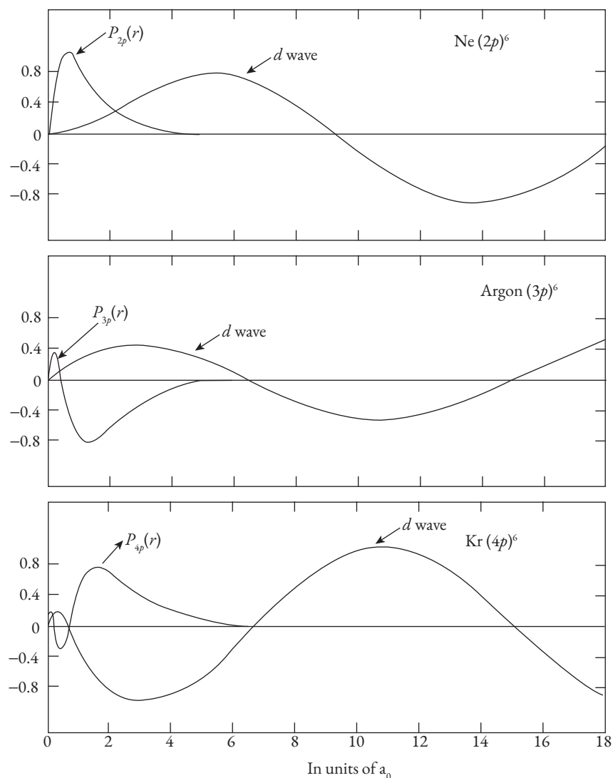
Fig. 5.3a The outermost 2p radial function in neon is nodeless, the argon 3p has one node, and the krypton 4p has two nodes. Also shown in each panel is the continuum d radial wavefunction at an energy that is just enough for ionization of the atom to take place on absorption of a photon. The photoelectron energy at the ionization threshold is \simeq 0 .
