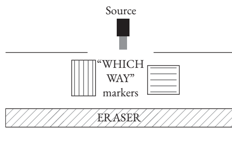
Fig. 3.2b In this arrangement, an additional polarizer is placed in the apparatus whose polarization axis is at 45^\circ angle with respect to that of the filter. This additional polarizer erases the WW information and restores interference.
