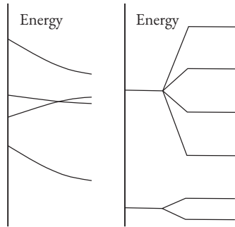
Fig. 6.3 As a result of a perturbation, the energy levels may change, and/or they may get split, in accordance with symmetry and conservation principles.
