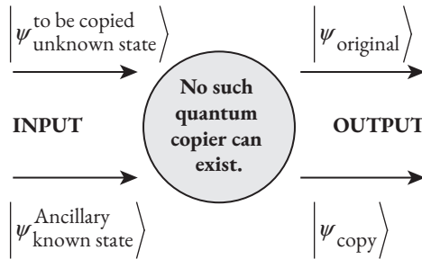
Fig. 11.13 We expect a quantum cloning machine to accept an arbitrary quantum state to be copied as input and copy it on an ancillary state and produce the original along with a copy of the original.
