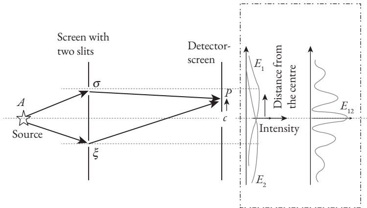
Fig. 2.1 The intensity vs. distance from centre C of the detector-screen is shown by the envelop E_1 when slit \sigma alone is open and by the envelop E_2 when slit \xi alone is open. It is shown by the envelop E_{12} when both the slits are open.
