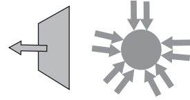
Fig. 10.5c This figure shows the plane wave moving from right to left. \cos(\theta + \pi) = -\cos\theta P_\ell(-\cos\theta) = P_\ell(\cos(\theta + \pi))
