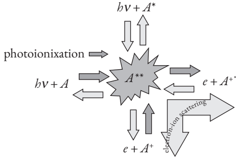
Fig. 10.2a This schematic diagram showing multiple pathways is based on Fig. 1.1 from Reference [4]. h\nu denotes a photon, e denotes an electron, A denotes a neutral atom and A^+ denotes a positive ion. An asterisk denotes an excited state.
