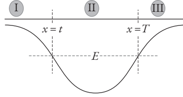
Fig. 6.2 A particle with energy E would be confined to region II, between the turning points t and T according to classical laws. The regions I and III are CF.
