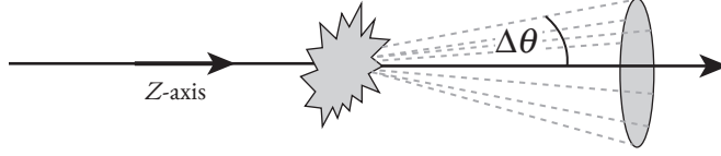
Fig. 10.7 The scatterer scoops out flux from the incident beam that would have continued its travel along the forward direction and spreads it in all the directions.
