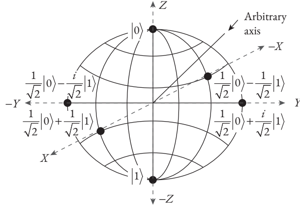
Fig. 11.6 Representation of a qubit according to Eq. 11.20 on a Bloch sphere. Qubit states on the intersection of the Cartesian coordinates and the Bloch sphere are explicitly labeled.
