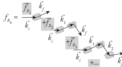
Fig. 10.14 Schematic representation of the Born series of multiple scattering (Eqs. 10.189a,b). Adapted from Chapter 8 of Reference [3].
