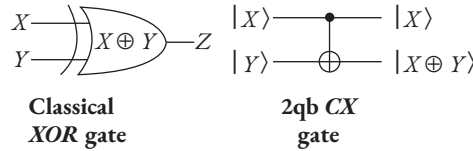
Fig. 11.9 The 2-qubit Control-Not gate is denoted using the symbol -\oplus- that denotes the classical XOR (exclusive OR) gate.
