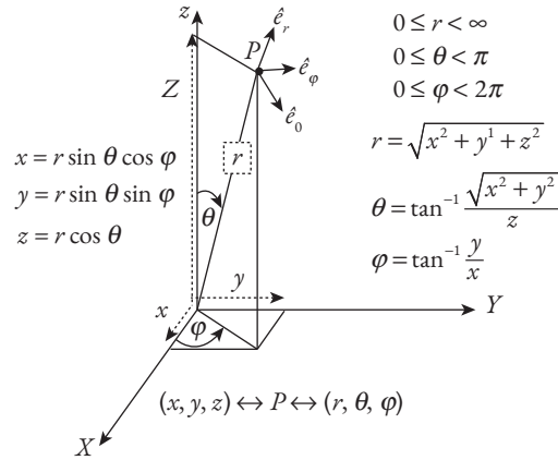
Fig. C.1 This figure shows the relationship between the Cartesian coordinate system and the spherical polar coordinates. The three Cartesian unit vectors \{\hat{e}_x, \hat{e}_y, \hat{e}_z\} are constant vectors along respective Cartesian axes. The unit vectors \{\hat{e}_r, \hat{e}_\theta, \hat{e}_\varphi\} of the spherical polar coordinate system at a typical point P are as shown in the figure. They point respectively in the direction of the increasing radial distance r , polar angle \theta , and the azimuthal angle \varphi . The notation is the same as in Reference [1].
