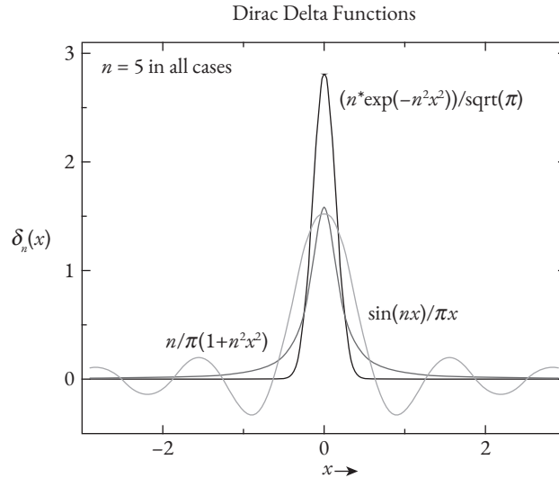
Fig. 6.4 The Dirac- \delta “function” is in fact better known as a distribution, or a generalized function. It is narrow and sharply peaked. There are various representations of the Dirac- \delta ; three of these representations are shown in this figure. Figures plotted by Jobin Jose.
