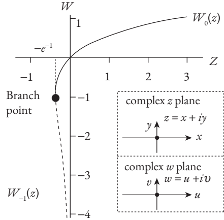
Fig. 3.11b The real branches W_0 and W_{-1} of the Lambert W function. W_0 is the principal branch.
