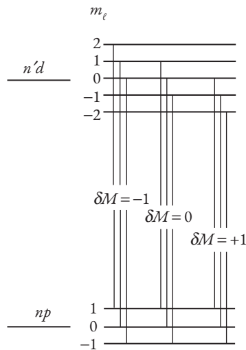
Fig. 8.8b The n'd \rightarrow np electric dipole line also splits into three spectral lines that are observed, which could also be explained away with no reference to the electron's spin.
