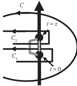
Fig. 5A.1 Contour chosen to avoid the singularities in the integrand in Eq. 5A.18. The flexed branch cut is also shown.
