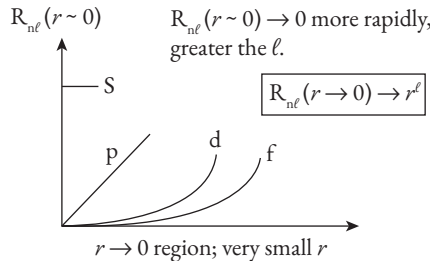
Fig. 5.1 Schematic depiction of the small- r ( r \rightarrow 0 ) behavior of the radial wave functions of the hydrogen atom.
