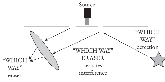
Fig. 3.3b A lens would recombine the scattered light from the two slits and erase the WW information. The quantum eraser restores interference.
