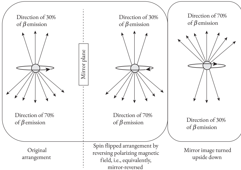
Fig. A.2a Parity violation in \beta -decay experiment.
