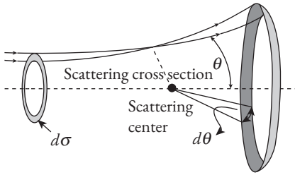
Fig. 10.1c The shaded ring on the left is in a flat plane, perpendicular to the direction of incidence. It is the same ring shown in Fig. 10.1b. The shaded strip on the right is on the surface of a sphere centered at the scatterer's center at a distance r .
