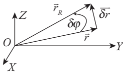
Fig. 4.2b In the rotation of a function, a point in the function at position \vec{r} is relocated to \vec{r}_R .
