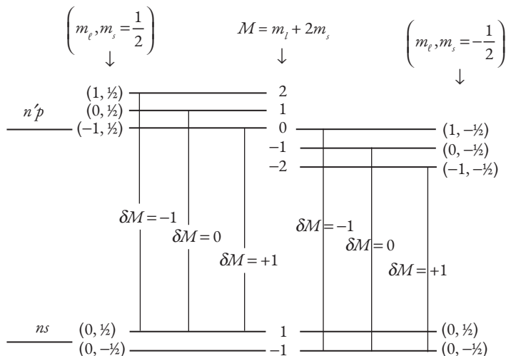
Fig. 8.7a The electric dipole transition n'p \rightarrow ns splits into six transitions, three of which correspond to m_s = +\frac{1}{2} and the other three to m_s = -\frac{1}{2} . Only three frequencies are, however, observed in the spectrometer since the splitting of the energy levels is equispaced.
