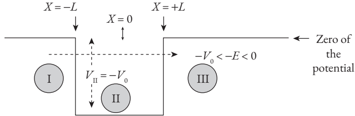
Fig. 3.7b One-dimensional potential well having a finite depth.
