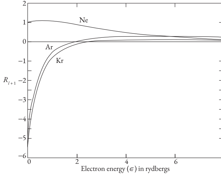
Fig. 5.3b The overlap between the initial state radial p ( \ell = 1 ) function and the final state radial d ( \ell = 2 ) function is shown in this figure as a function of the photoelectron energy. It is always positive in the case of neon, but in the case of argon and krypton the sign changes, going through a zero at a particular photoelectron energy where the Cooper minimum occurs.
