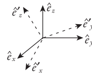
Fig. 4.2c The rotation of a function can also be described from a passive point of view in which the coordinate frame itself is rotated in the opposite rotation.
