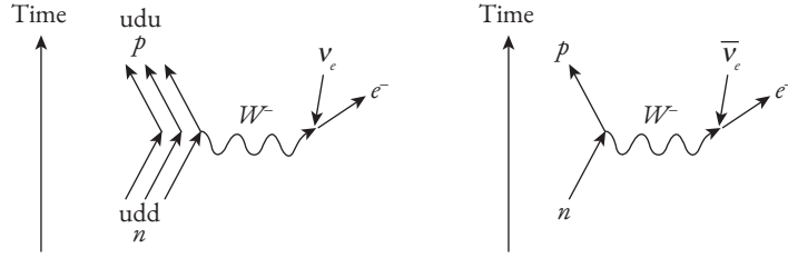
Fig. A.1 A neutron ( n ) is a spin-half baryon. It consists of three quarks, up, down, down. The weak interaction mediated by W^- boson transforms it into a proton ( p ) which consists of the three quarks up, down, up. An electron and an antineutrino (electron-antineutrino) are emitted.
