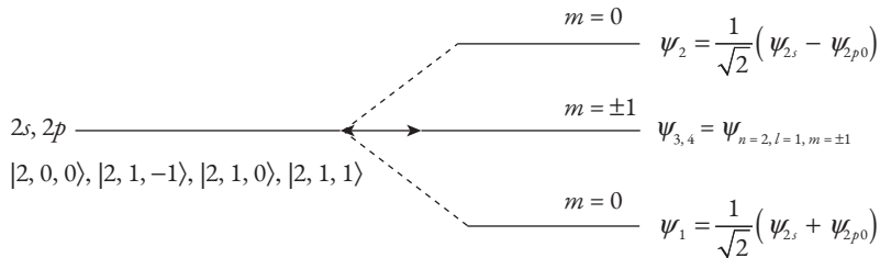
Fig. 8.5 First-order Stark effect for n = 2 , the first excited state of the hydrogen atom. The energy splitting is E_{n=2}^{(1)} = \mp (3e a_0 \times \epsilon) .
