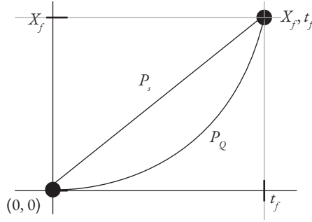
Fig. 2.3 Schematic diagram showing one-dimensional motion along the (vertical) x -axis against the (horizontal) time axis. A free particle's motion from (x_i = 0, t_i = 0) to (x_f, t_f) . Newton's method provides the correct path P_s (straight line). Consideration of variations in the quadratic path P_Q explains why the classical trajectory turns out to be correct.
