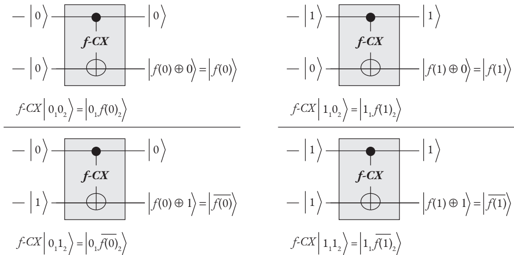
Fig. 11.11a Depicting the operations in Eqs. 11. 38a,b. Fig. 11.11b Depicting the operations in Eqs. 11. 38c,d.
