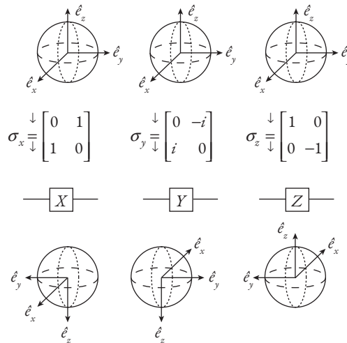
Fig. 11.7 Rotation of the Bloch sphere under the Pauli-X, -Y, -Z gates.
