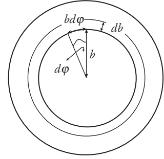
Fig. 10.1b Different parts of the incident particles are at different impact parameter distances from the scatterer's center. The scattering process is considered to have cylindrical symmetry about the Z -axis, independent of the azimuthal angle \phi .
