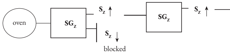
Fig. 1.2b This experiment shows that a mixed state collapses into an eigenstate by a measurement. Furthermore, a system that is produced in an eigenstate (in this case by the first SG apparatus) remains in the same eigenstate if the same measurement is repeated.
