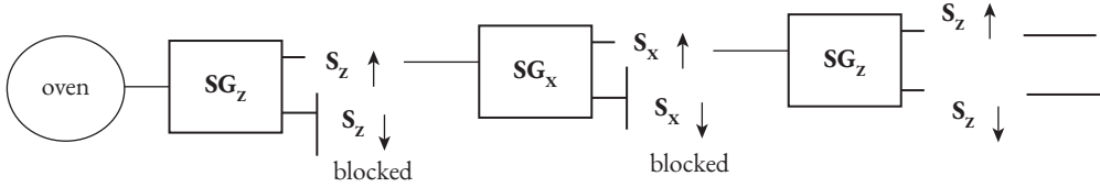
Fig. 1.2d This sequential SG experiment shows that measurements of Z - and X -components of the magnetic moment are not compatible with each other.
