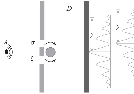
Fig. 2.5c The Aharonov–Bohm experiment is essentially a Young’s double-slit experiment in which a solenoid is placed right behind the slits and in between them. The solenoid is impenetrable, so electron trajectories can only skirt the solenoid on either side. The shaded circle right behind the slits shows the top view of the solenoid.
