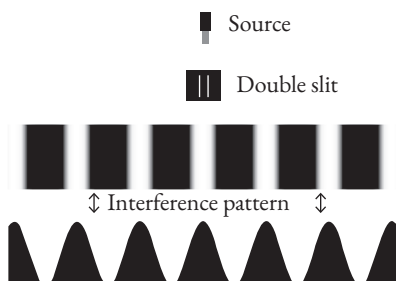
Fig. 3.1 Schematic representation of interference between alternatives resulting in bright and dark fringes.
