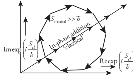
Fig. 2.4 When S \gg \hbar , paths nearby to the classical paths add up in phase; those away from the same cancel each other.
