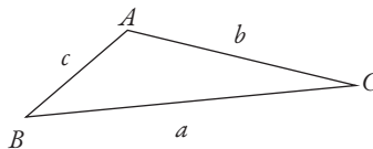
Fig. 4.4 Lengths of the three sides of a triangle satisfy the triangle inequality |c - a| \leq b \leq (a + c) .
