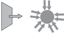
Fig. 10.5a The Z-axis is assumed pointed from left to right. This figure shows the plane wave moving along the positive Z-axis.
