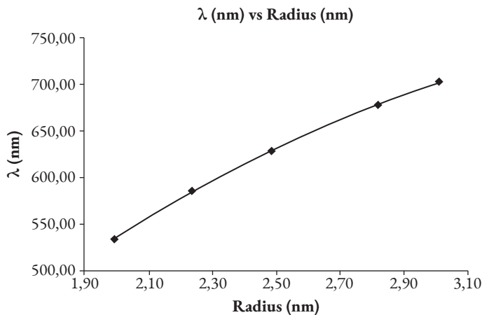
Fig. 3.10a Optical properties of a quantum dot are related to its size.
