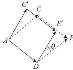
Fig. P8.2 In the first experiment with the neutron interferometer, we consider the case when the plane ADECA is horizontal. We then raise the arm CE to C'E' by turning the interferometer through an angle \theta about the arm AD . The track C'E' is now at a height DE\sin\theta higher than the arm AD . Note that DE = DE' .
